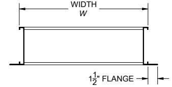
MODEL: 2625 FRAME: FLANGE FRAME FLANGE-MOUNT (FM)
