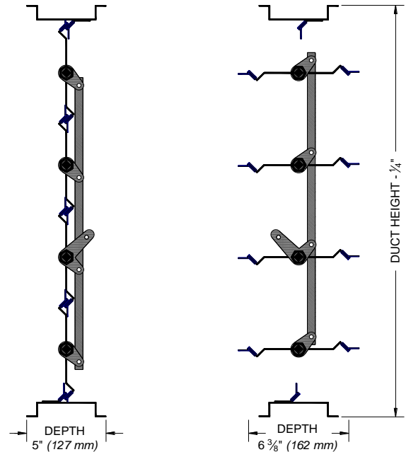
4100-304SS Stainless Steel, Low Leakage Control Damper
