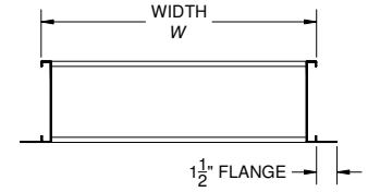
MODEL: 2625 FRAME: FLANGE FRAME FLANGE-MOUNT (FM)
